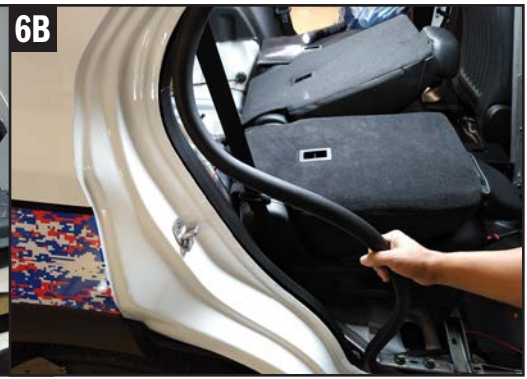
6 · Pop loose the (2) press in pins holding the panel to the lower seat skirt fabric, remove trim section. · Fold the rear seats down and pull the rubber door seal away from the "C-Pillar" side panel.
