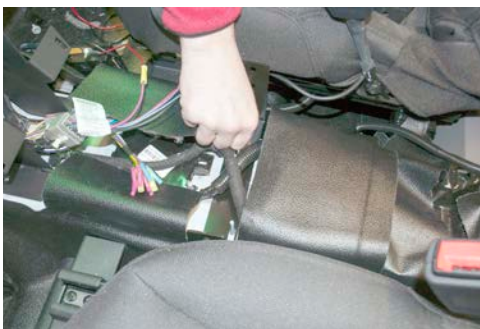
Slide Rear Mount Bracket under OEM wiring. Secure using the supplied (2) M6-1.0 x 25 bolts.
