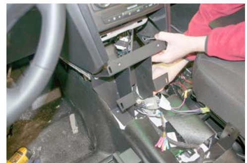
Place Jotto Desk Forward Mount Bracket into OEM Dash.
