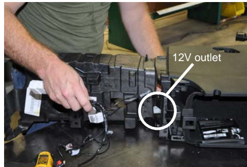
Now, with all components out of OEM console, remove any remaining wiring and 12V outlet from inside storage box. Set aside OEM console substructure.
