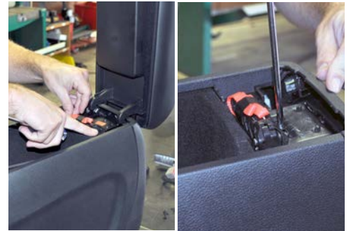
To remove Manual Park Release, you will need to remove (3) Phillips screws and set arm rest aside. Then remove (2) Phillips screws that are exposed.
