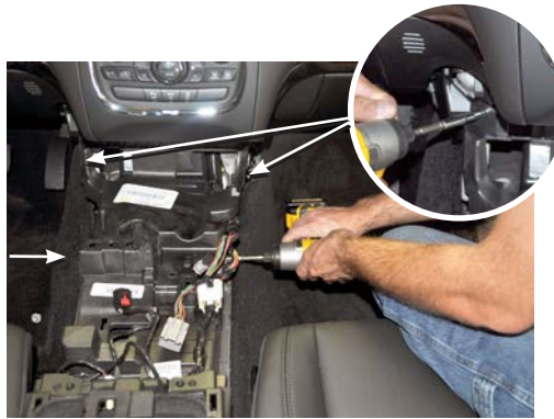
Remove (2) 10mm bolts and (2) 7mm bolts.
