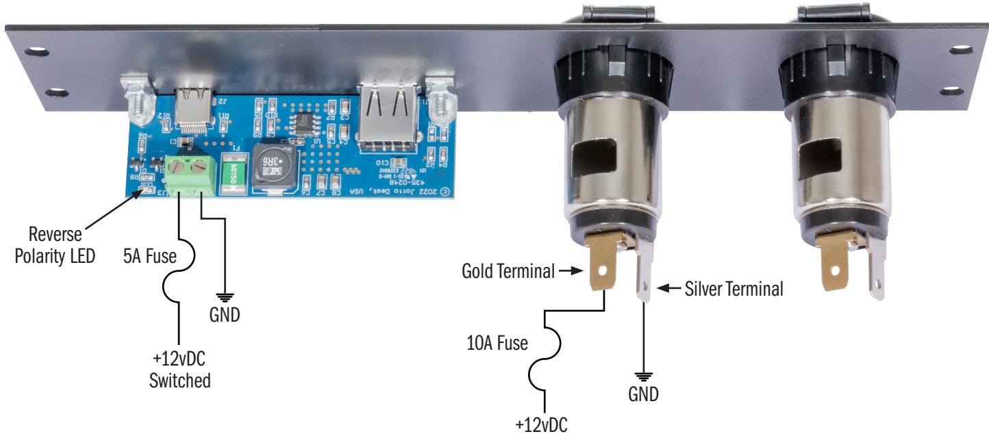
USB Board
