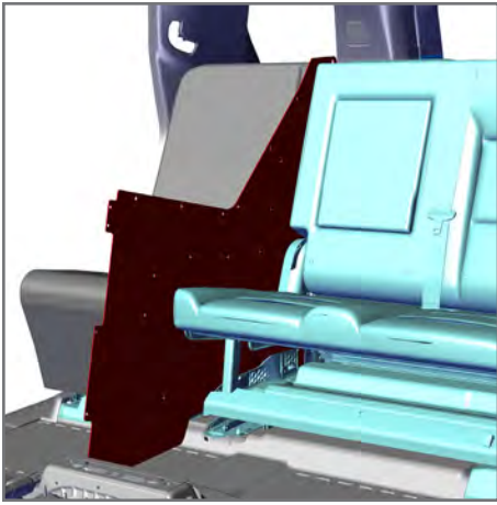
16. Slip the Lower Steel Center Divider between split in rear seats.
