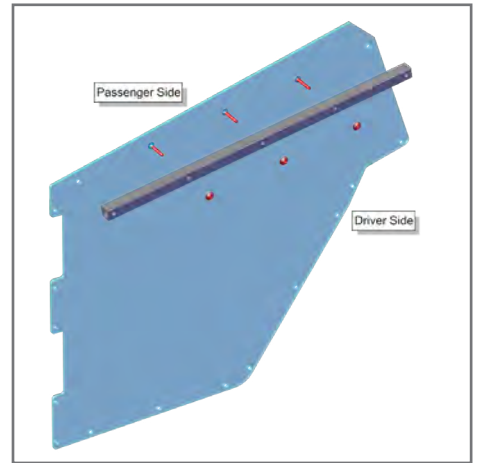
21. Outside of vehicle, attach the Stiffener Tube to the D/S Upper Poly Center Divider with provided carriage bolts and flange nuts.
