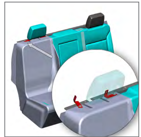
15. Push the top of the ABS Seat through the headrest supports. This may require simple adjustments of the previously mounted ABS Seat Brackets.
