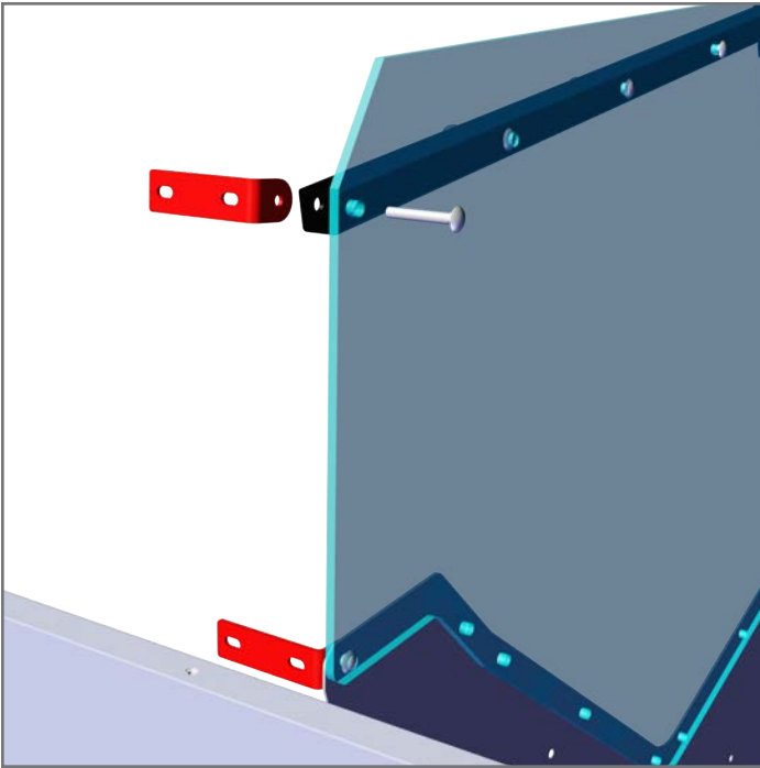
19. Attach the Secure Grid Bracket to the end of the Stiffener Tube and Lower Steel Divider with provided carriage bolts and flange nuts.
