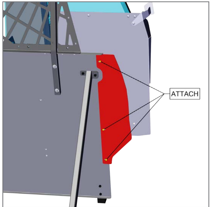
22. Install Lower DS/PS Side Wings with provided hex bolts and washers to the rear side of the Steel Panel.
