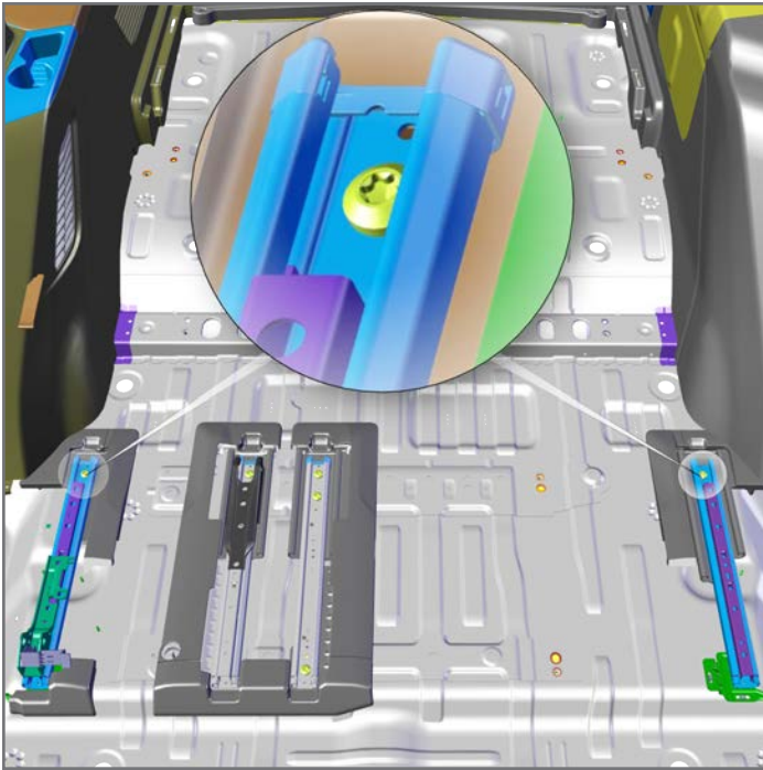
1. Fold both sections of rear seat down and tilt forward. Loosen outer most rear OEM seat bolts.
