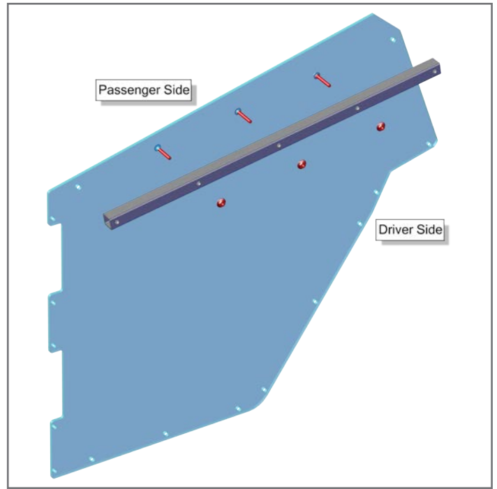
16. Outside of vehicle, attach Stiffener Tube to Upper Poly Center Divider with provided carriage bolts and flange nuts.
