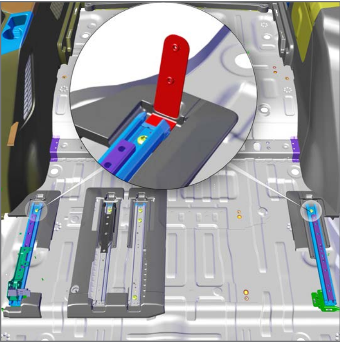
2. Loosely install the DS/PS Lower Mount Brackets under the seat frame.
