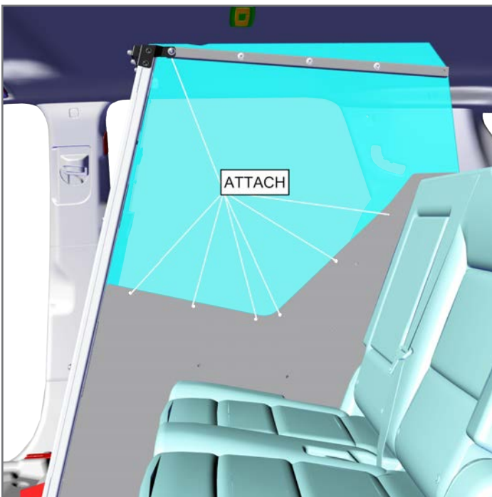
17. Attach Upper Poly Center Divider to Lower Steel Center Divider and Assembled Front Divider from P/S side using provided carriage bolts and flange nuts. Loosely tighten all bolts at this time.
