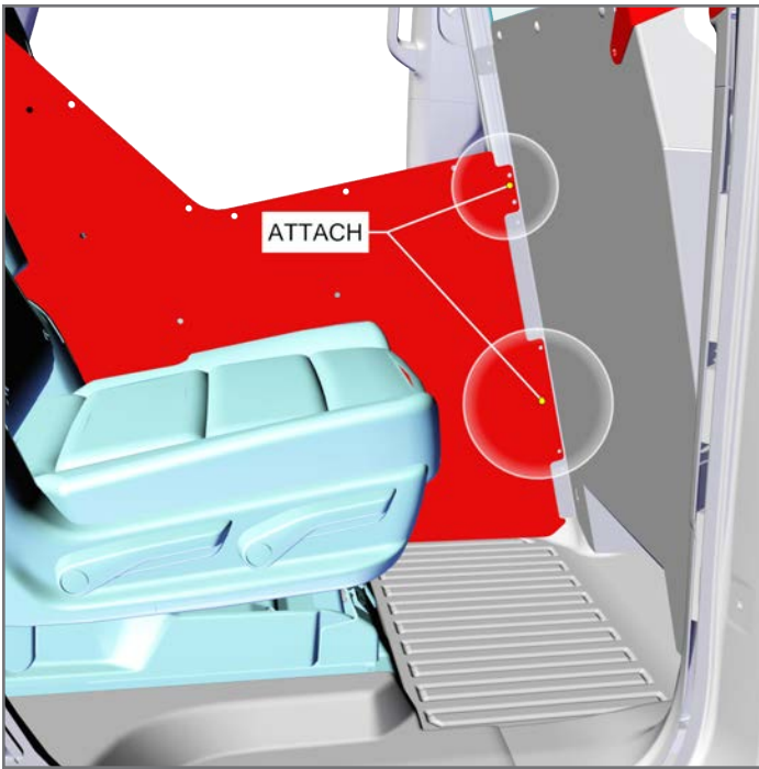
15. Loosely secure Lower Steel Center Divider onto Assembled Front Divider to the pre-positioned T-Blocks located in the rail of the Extruded Backbone with provided socket head cap screws.
